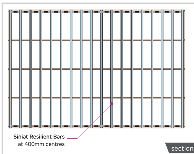
FC-DT-102-Timber frame layout with Siniat Resilient Bars
